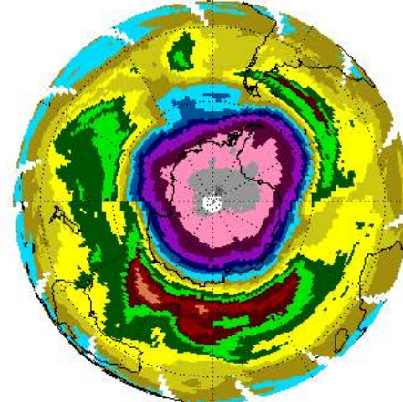
EP/TOMS Total Ozone for Oct 1, 1999
