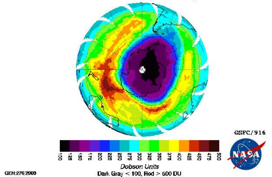
EP/TOMS Total Ozone for Oct 1, 2003
