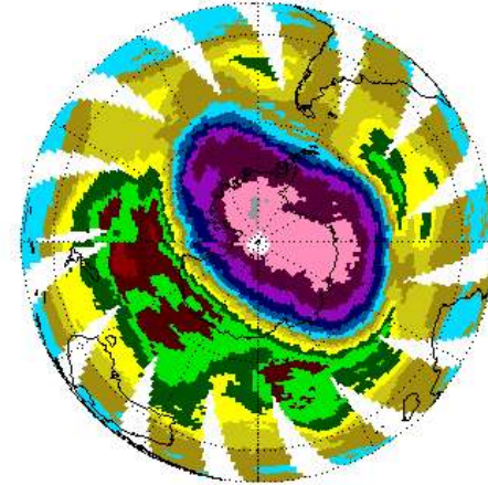
EP/TOMS Total Ozone for Oct 1, 1997
