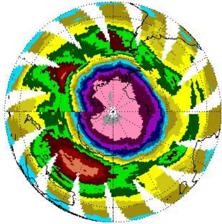
EP/TOMS Total Ozone for Oct 1, 1996
