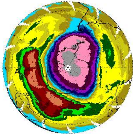
EP/TOMS Total Ozone for Oct 1, 1998
