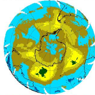
EP/TOMS Total Ozone for Feb 1, 2000
