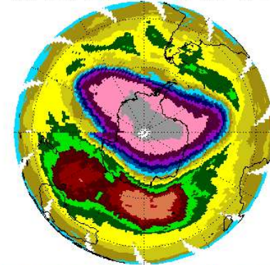
EP/TOMS Total Ozone for Oct 1, 2000
