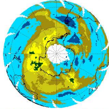
EP/TOMS Total Ozone for Apr 1, 2000
