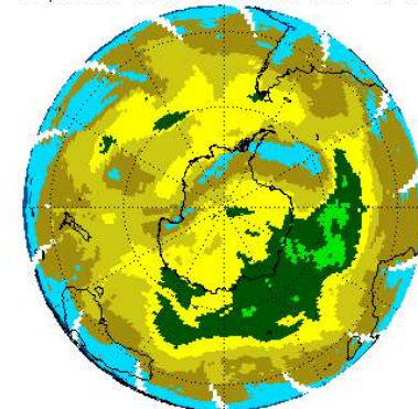
EP/TOMS Total Ozone for Dec 1, 2000
