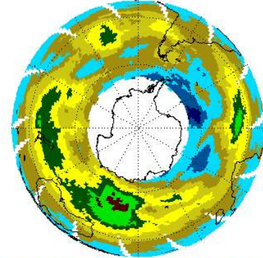
EP/TOMS Total Ozone for Aug 1, 2000
