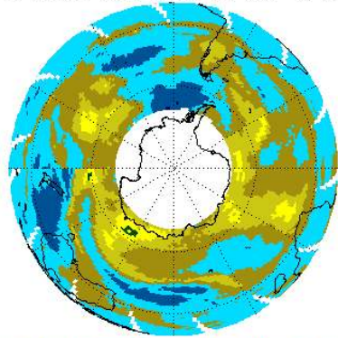
EP/TOMS Total Ozone for May 1, 2000
