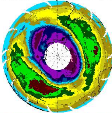
EP/TOMS Total Ozone for Sep 1, 2000
