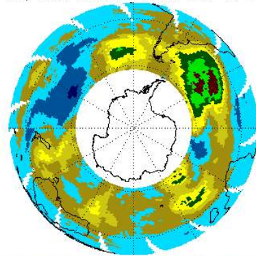
EP/TOMS Total Ozone for Jun 1, 2000
