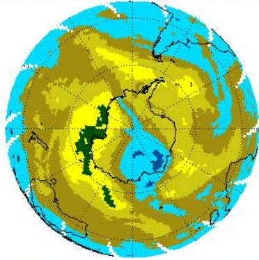
EP/TOMS Total Ozone for Jan 1, 2000
