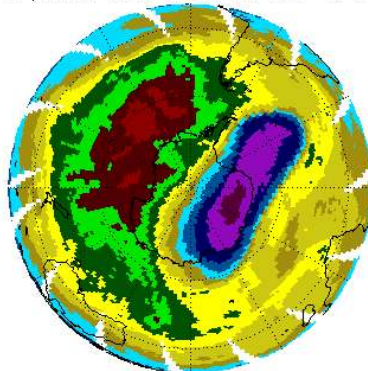
EP/TOMS Total Ozone for Nov 1, 2000
