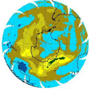
EP/TOMS Total Ozone for Mar 1, 2000
