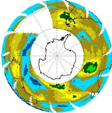
EP/TOMS Total Ozone for Jul 1, 2000
